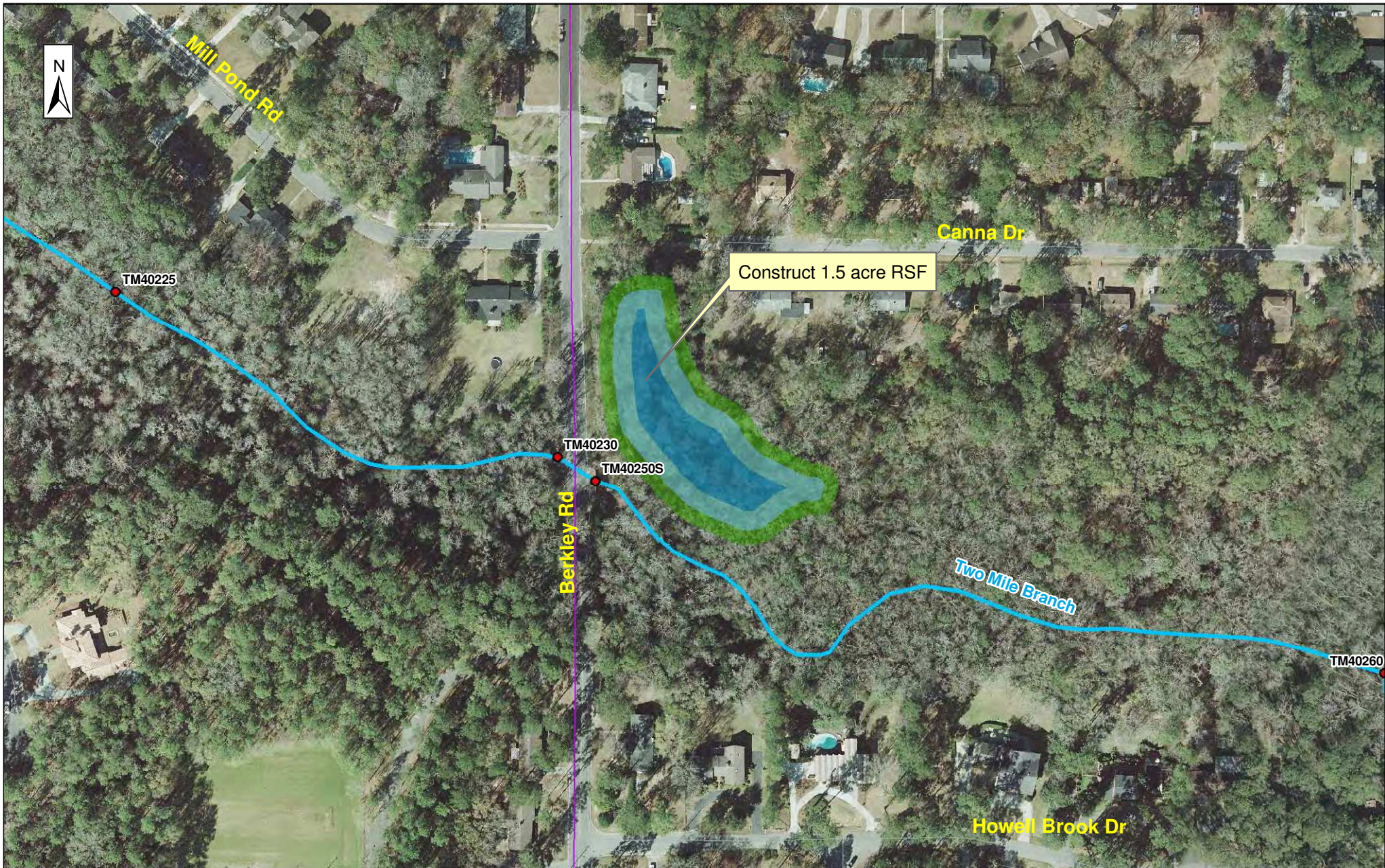
Figure 4.6.5 City of Valdosta, GA Two Mile Branch Sub-basin Alternative TM3 Regional Stormwater Facility near Berkley Road
