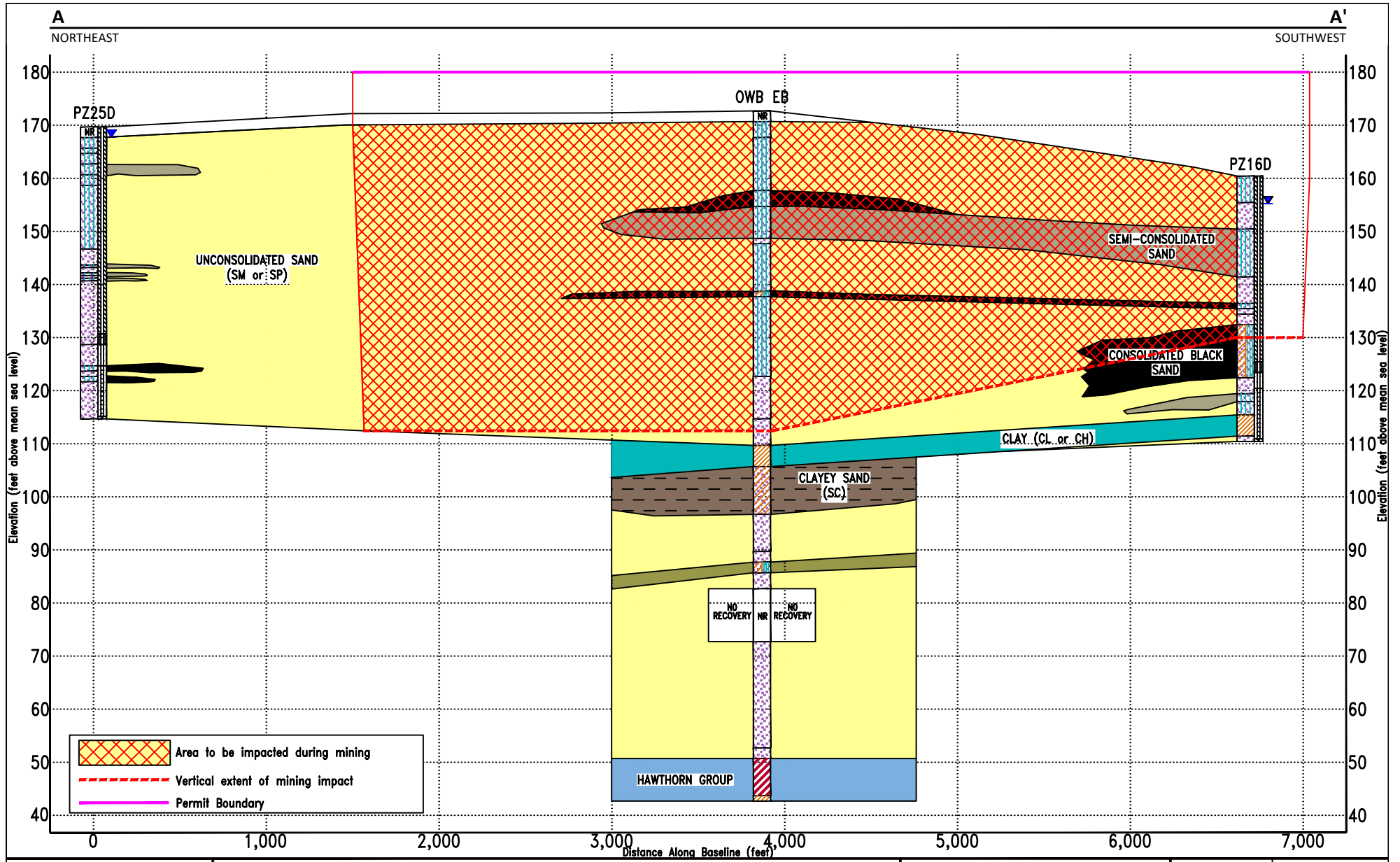
Figure 2. Generalized Hydrogeologic Cross-Section A - A' Twin Pines Minerals USACE Individual Permit Application St. George, Charlton County, Georgia
