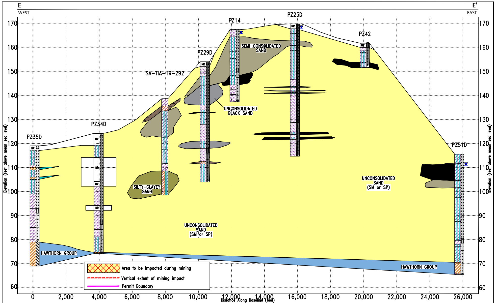
Figure 5. Generalized Hydrogeologic Cross-Section E - E' Twin Pines Minerals USACE Individual Permit Application St. George, Charlton County, Georgia
