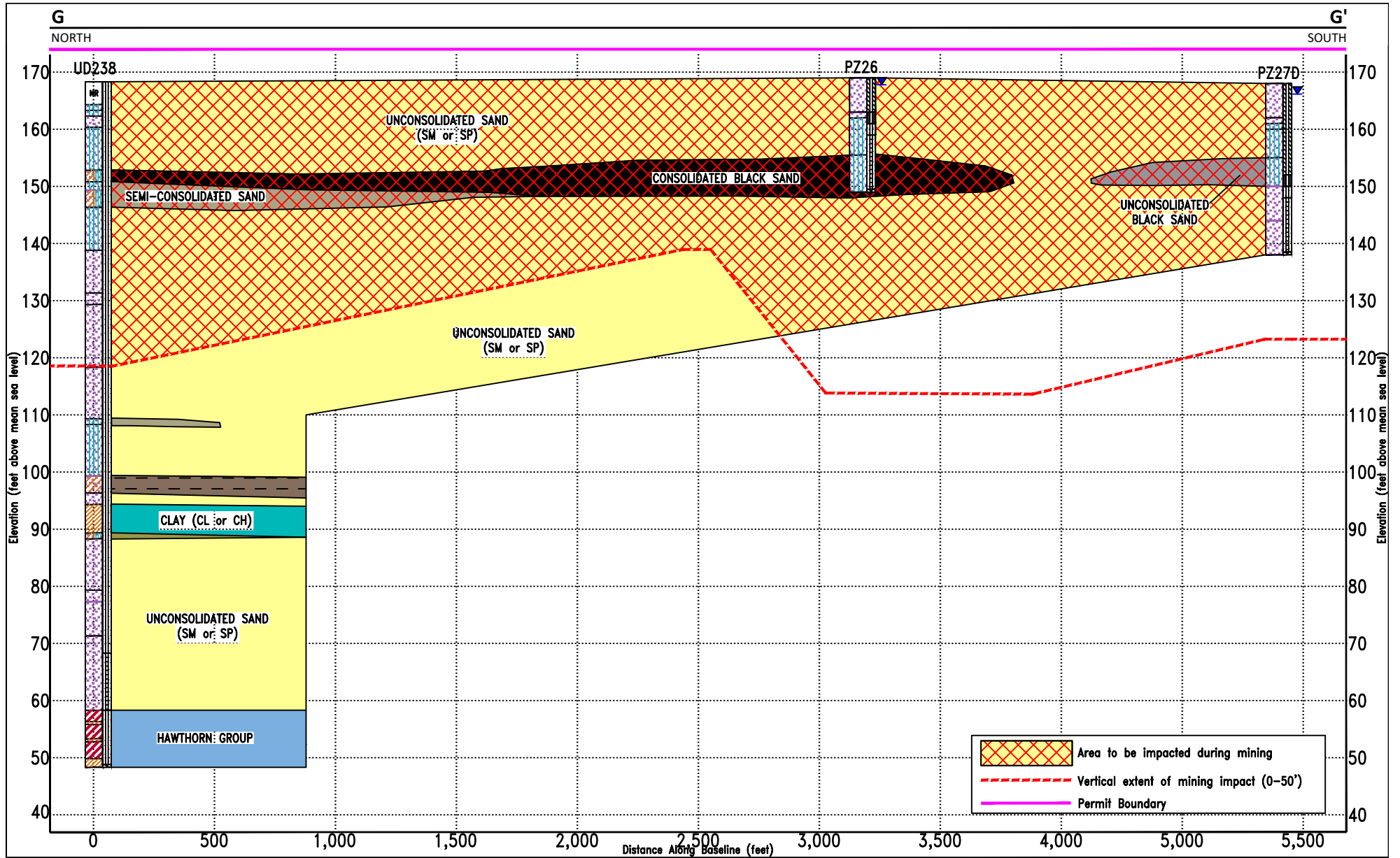
Figure 6. Generalized Hydrogeologic Cross-Section G - G' Twin Pines Minerals USACE Individual Permit Application St. George, Charlton County, Georgia
