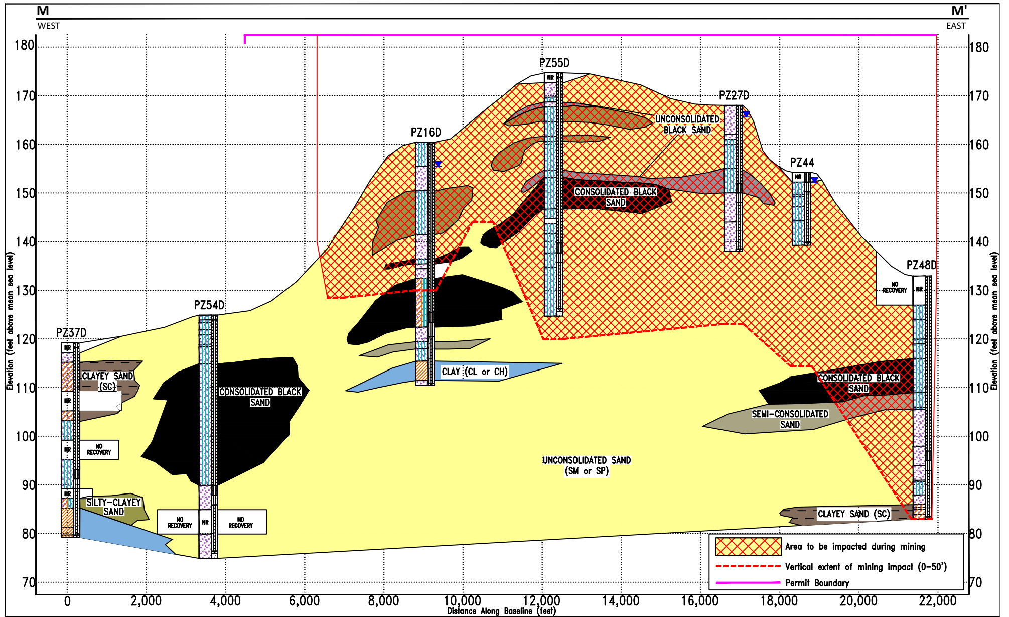
Figure 10. Generalized Hydrogeologic Cross-Section M - M' Twin Pines Minerals USACE Individual Permit Application St. George, Charlton County, Georgia
