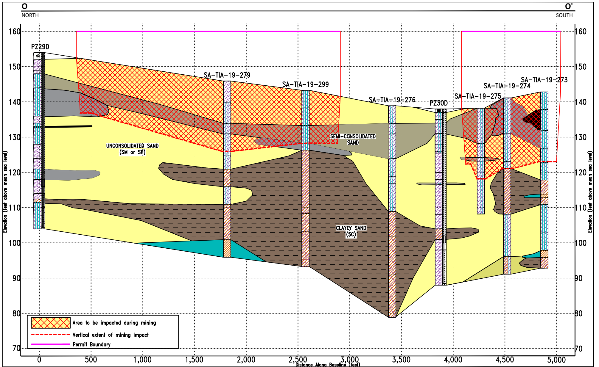
Figure 11. Generalized Hydrogeologic Cross-Section O - O' Twin Pines Minerals USACE Individual Permit Application St. George, Charlton County, Georgia
