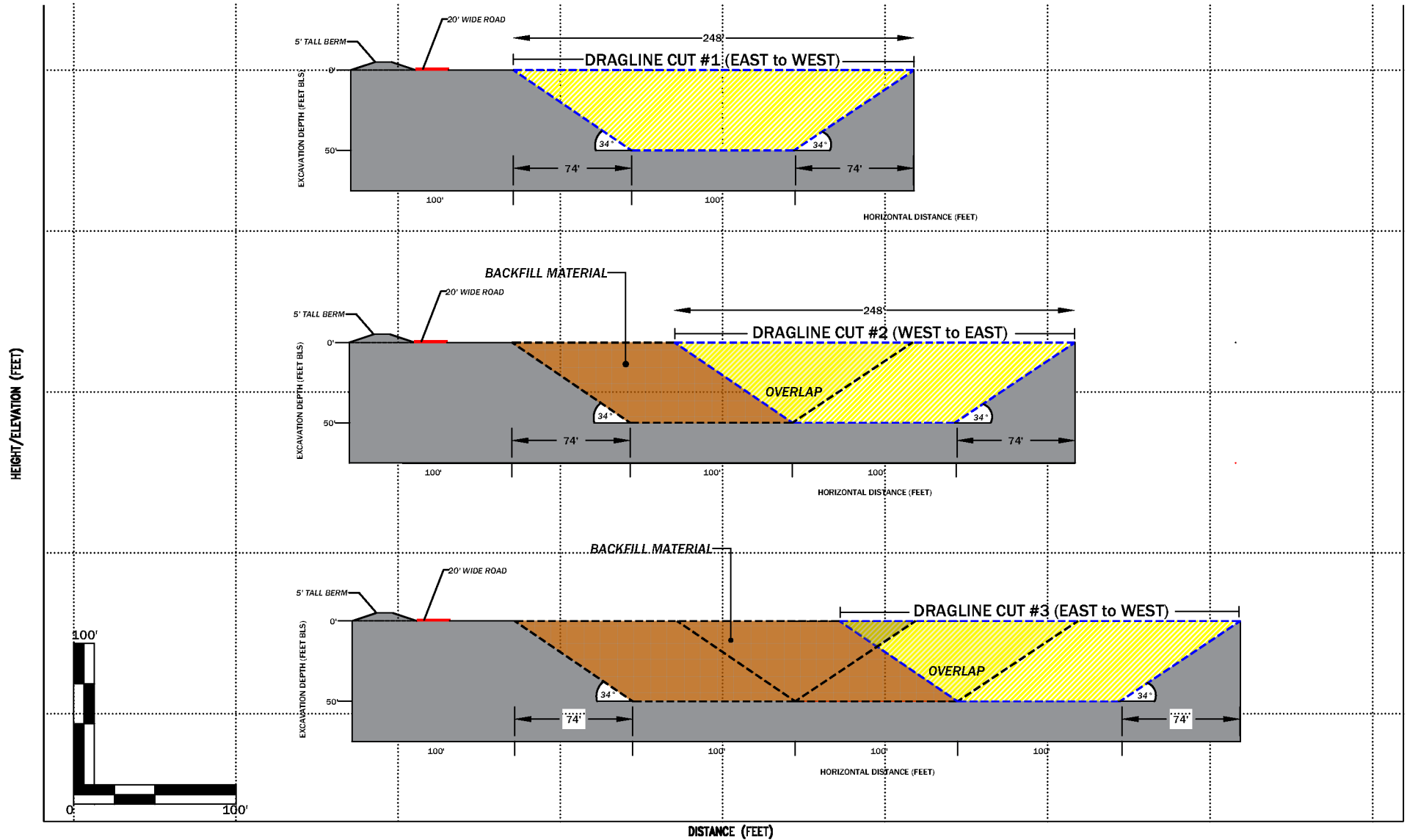
Figure 6. Impact Excavation Design Cross-Section Z - Z' Twin Pines Minerals USACE Individual Permit Application St. George, Charlton County, Georgia
