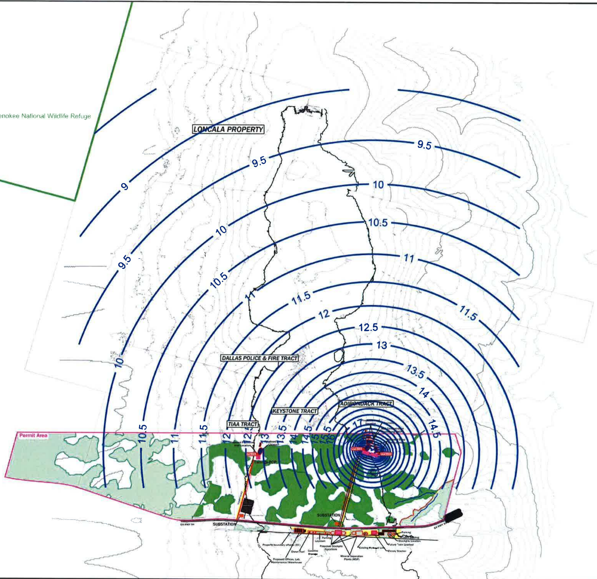
SITE MAP SHOWING PUMPING WELL BASE DRAWDOWN AT 1825 DAYS TWIN PINES MINERALS ST. GEORGE, CHARLTON COUNTY, GEORGIA
