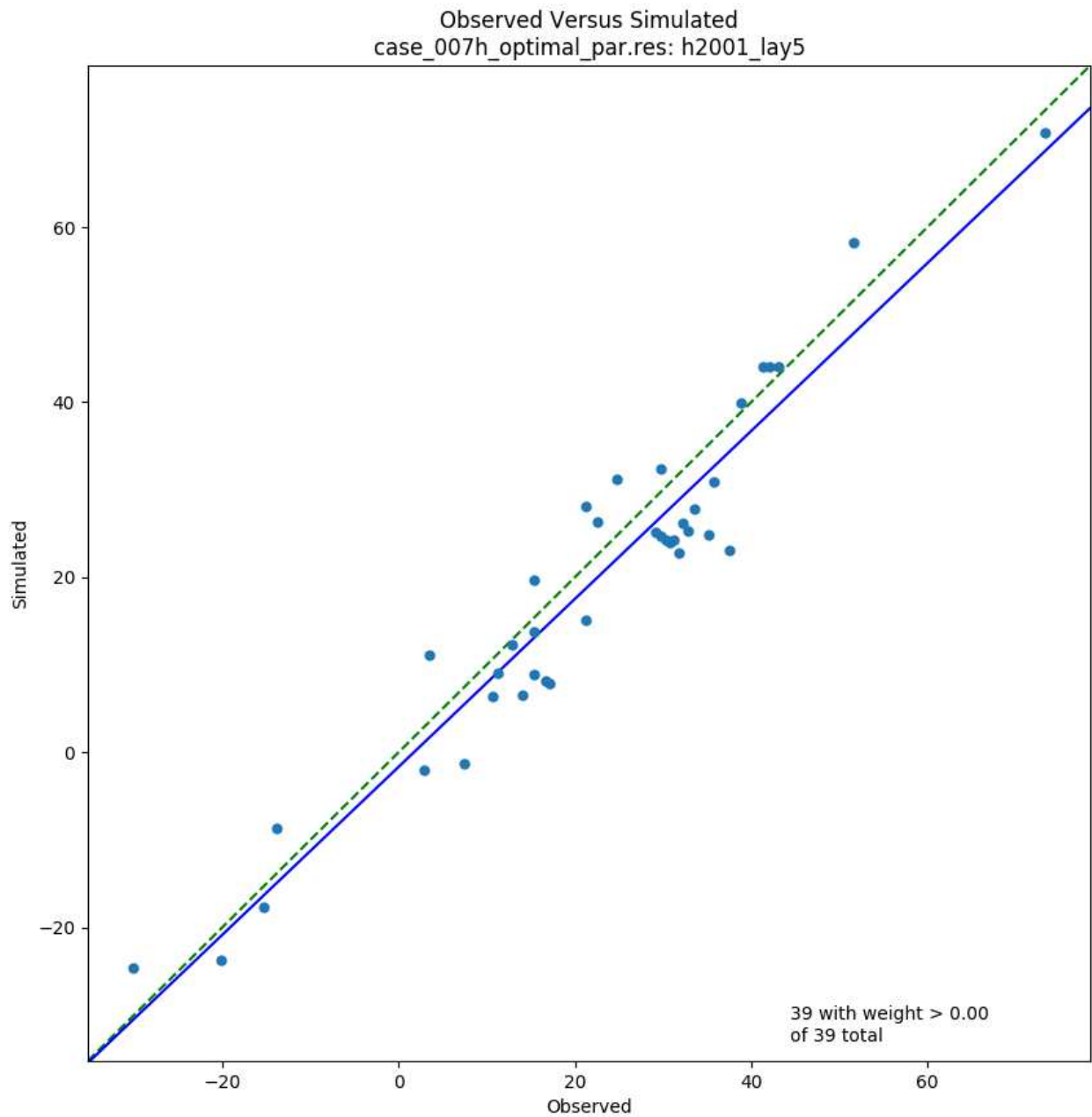
Figure 4-37. Observed versus simulated hydraulic head (feet NAVD88), model Layer 5, 2001
