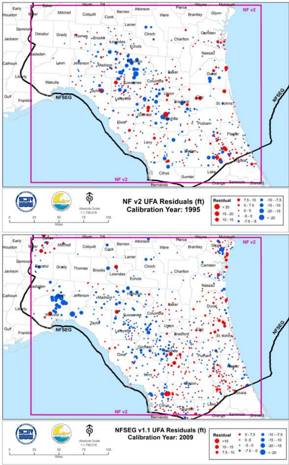
Figure 4-83. Residuals of UFA hydraulic head (feet), North Florida Model Version 2 and NFSEG v1.1 (2009)
