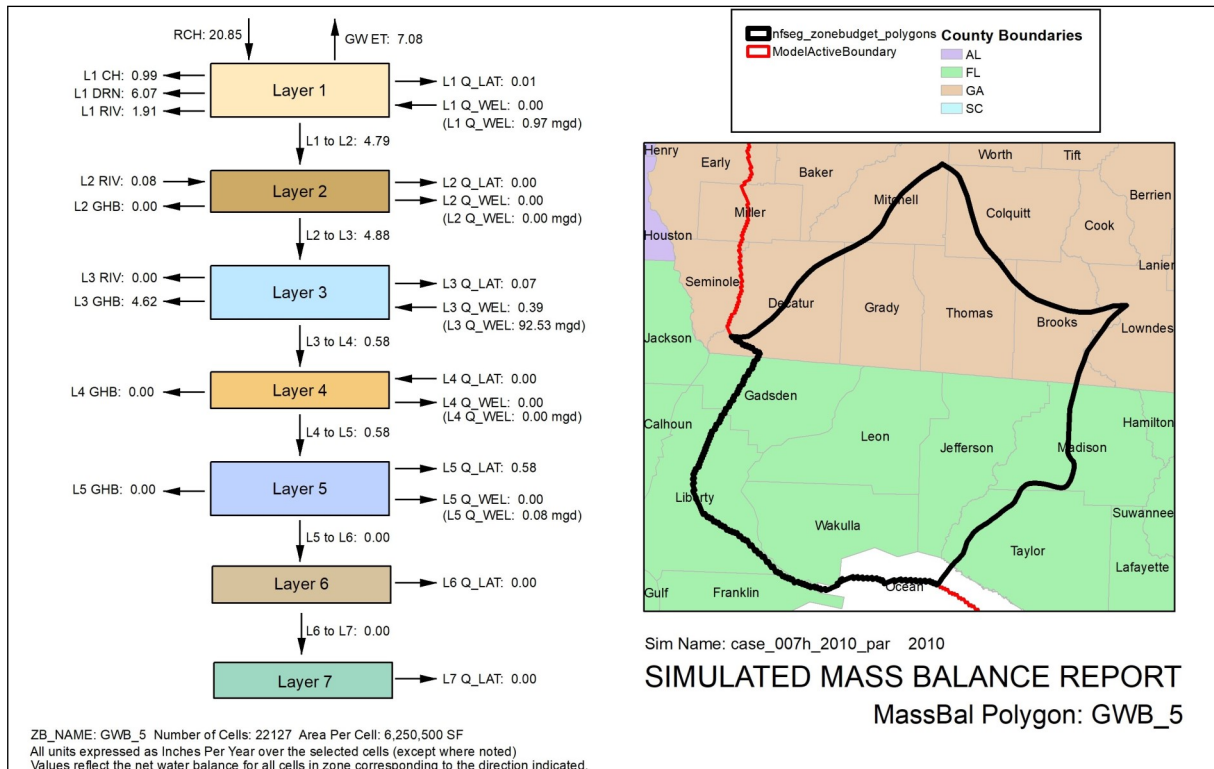
Figure 6-24. Simulated mass balance of GWB 5 for 2010
