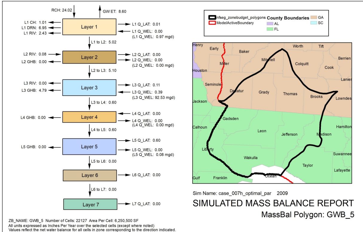
Figure 6-23. Simulated mass balance of GWB 5 for 2009
