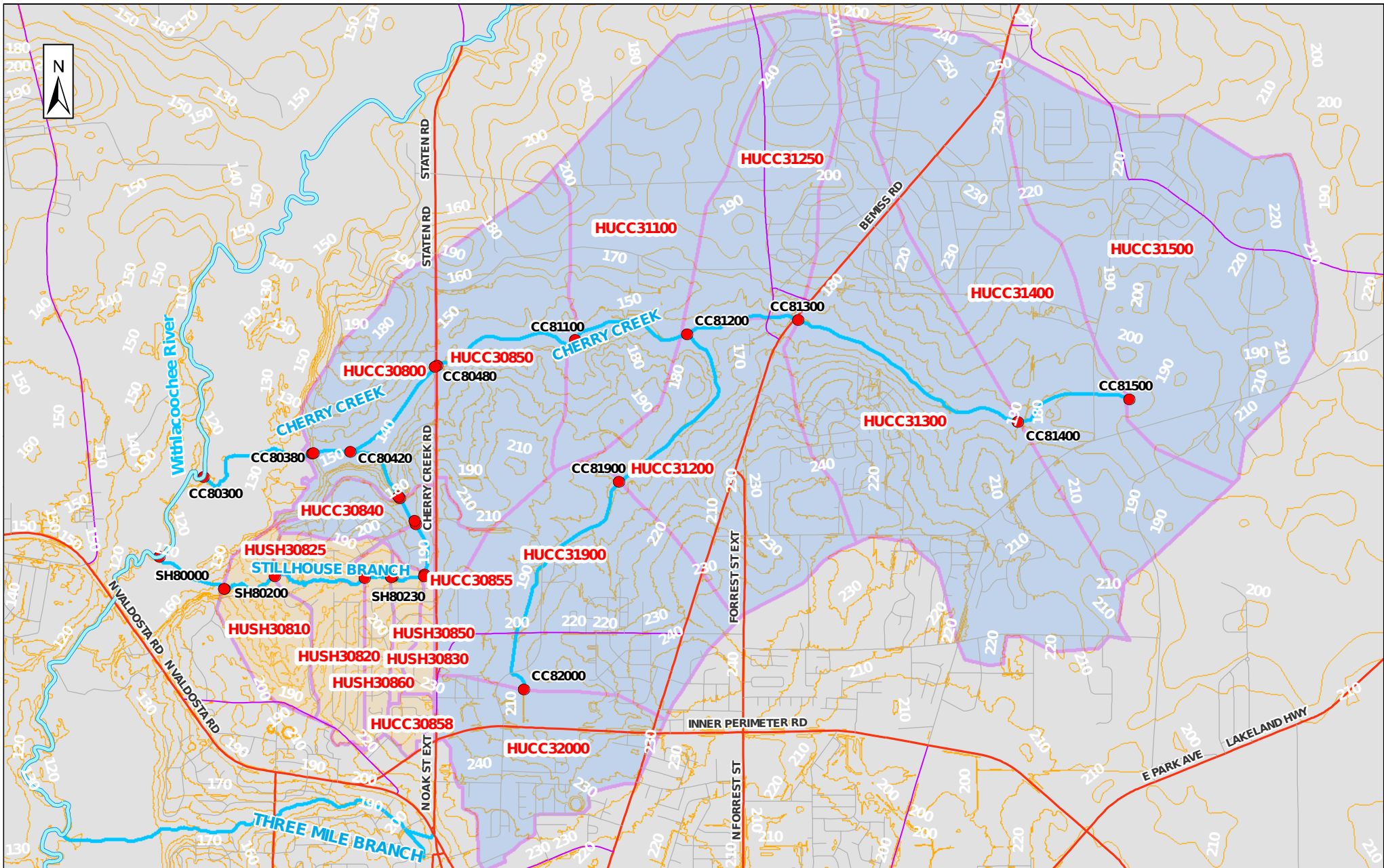
Figure 4.2.2.1 City of Valdosta, GA Cherry Creek Sub-Basin Stillhouse Branch Sub-Basin Hydraulic Network
