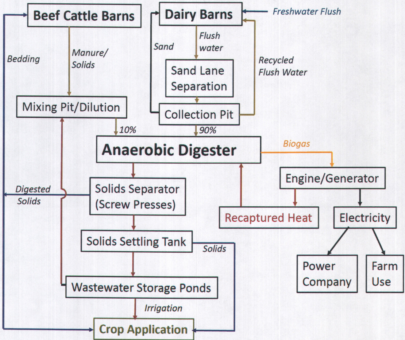
Figure 7. Flow Diagram of Waste Management and Bio Energy System
