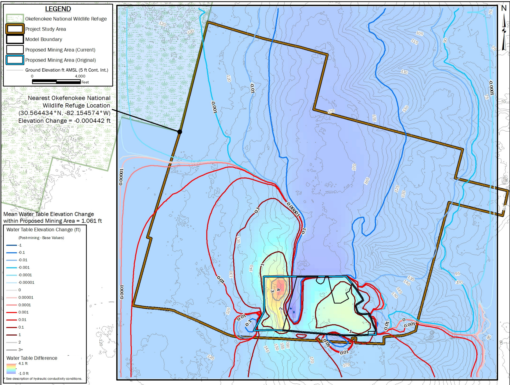
FIGURE 28: HYDRAULIC HEAD DIFFERENCE BETWEEN LAYERED SCENARIO HERE MODELED HERE & PRE-MINING SCENARIO OF HOLT ET AL. (2020); THE VERTICAL EFFECTIVE K OF THE UPPER 10 FEET OF THE MINE FOOTPRINT IS 1E-06 CM/S & THE HORIZONTAL K IS 1E-03 CM/S TWIN PINES MINERALS, LLC SAUNDERS DEMONSTRATION MINE ST. GEORGE, CHARLTON COUNTY, GEORGIA
