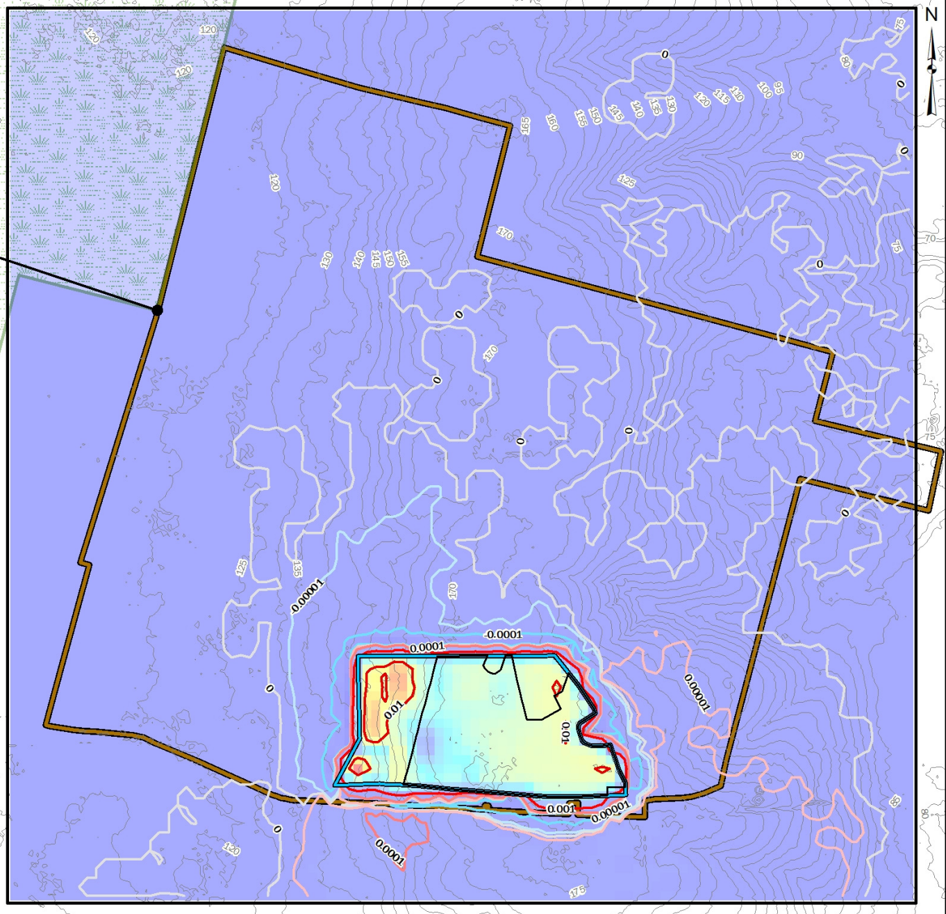
FIGURE 18: HYDRAULIC HEAD DIFFERENCE BETWEEN LAYERED SCENARIO HERE MODELED HERE & POST-MINING SCENARIO OF HOLT ET AL. (2020); THE VERTICAL EFFECTIVE K OF THE UPPER 10 FEET OF THE MINE FOOTPRINT IS 1E-04 CM/S & THE HORIZONTAL K IS 1E-03 CM/S TWIN PINES MINERALS, LLC SAUNDERS DEMONSTRATION MINE ST. GEORGE, CHARLTON COUNTY, GEORGIA
