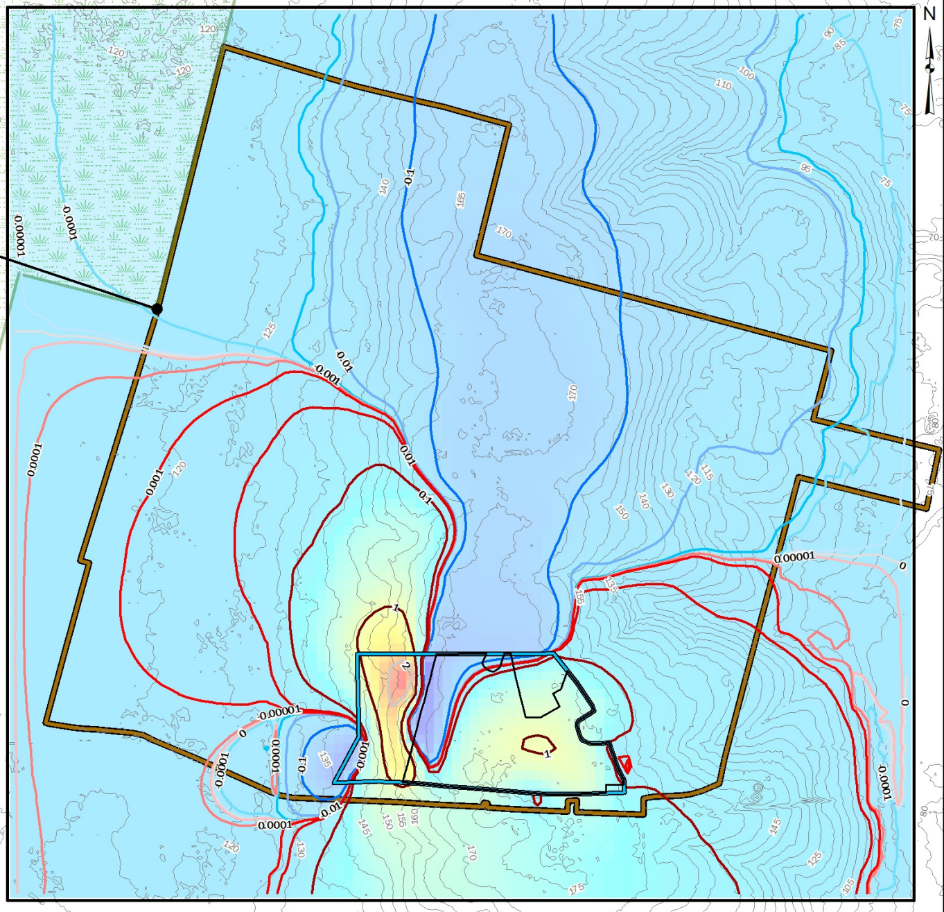
FIGURE 23: HYDRAULIC HEAD DIFFERENCE BETWEEN HOMOGENEOUS SCENARIO MODELED HERE & PRE-MINING SCENARIO OF HOLT ET AL. (2020); THE VERTICAL & HORIZONTAL K OF THE UPPER 10 FEET OF THE MINE FOOTPRINT IS 1E-05 CM/S TWIN PINES MINERALS, LLC SAUNDERS DEMONSTRATION MINE ST. GEORGE, CHARLTON COUNTY, GEORGIA
