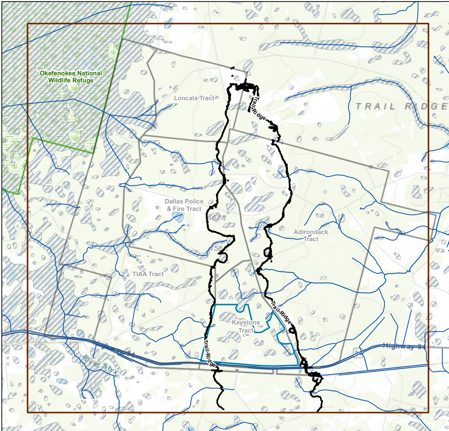
Figure 22 National Hydrography Dataset Delineated Wetlands and Stream Channels in Study Area
