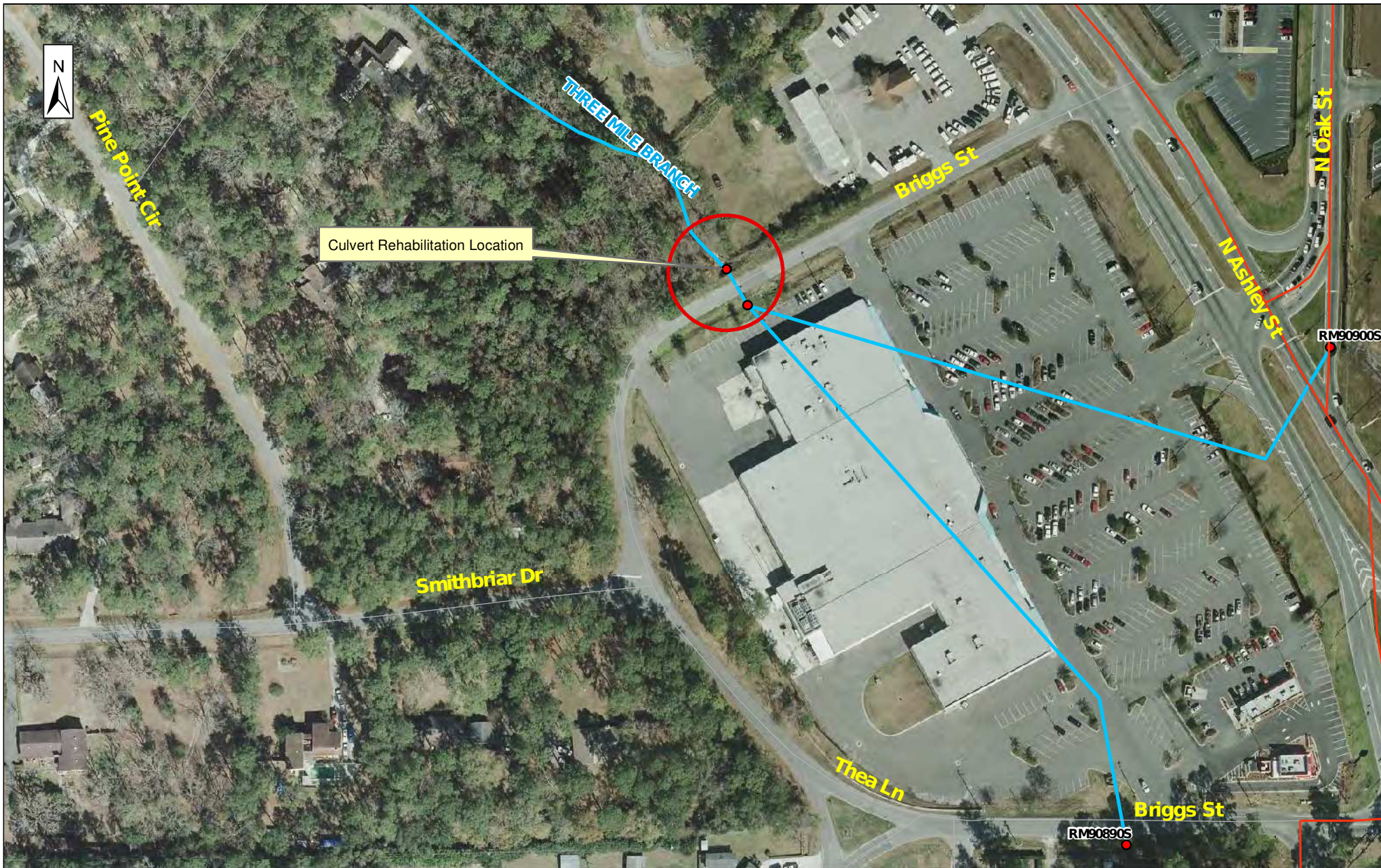
Figure 4.7.5 City of Valdosta, GA Three Mile Branch Sub-Basin Alternative RM3 Briggs Street Culvert Rehabilitation
