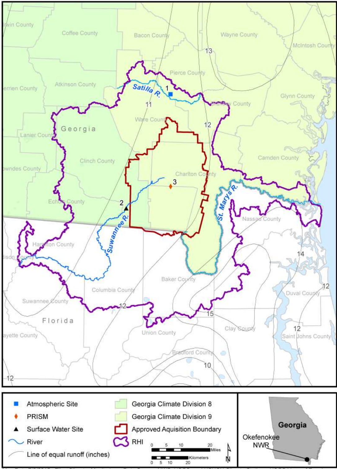
Figure 10. Climate monitoring stations, Georgia Climate Divisions, and lines of annual equal runoff for the Okefenokee National Wildlife Refuge Region of Hydrologic Influence (RHI). Numbered sites are listed in Table 4.
